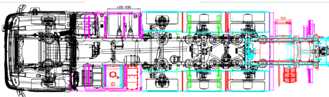
Pusher-tridem WB4900
